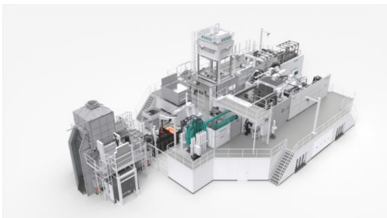
Carat 720 megacasting cell
